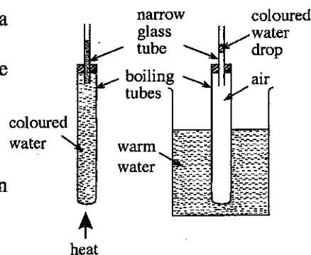
Set-up A
